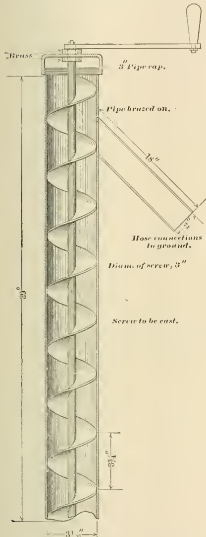
ARRANGEMENT FOR LOWERING SAND.
